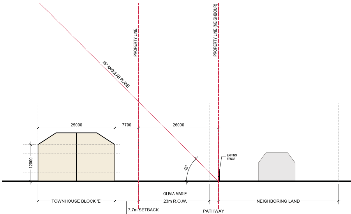
Angular Plane Cross-Section of Townhouse Block 'E'
