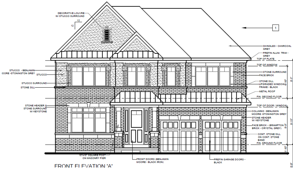
Conceptual Elevation of a single detached dwelling
