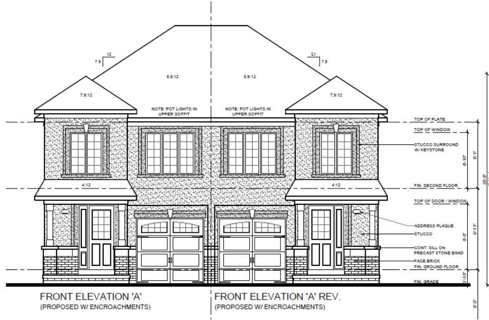
Conceptual Elevation of a semi-detached dwelling
