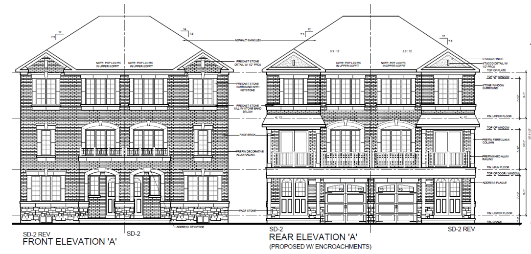
Conceptual Elevation of a dual frontage semi-detached dwelling
