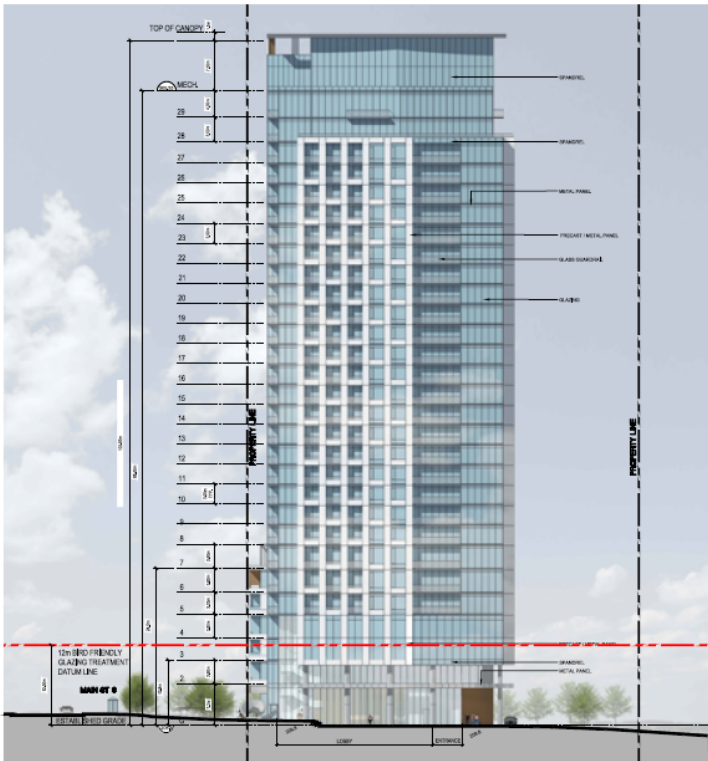
South Elevation (Bartley Bull Parkway Frontage)
