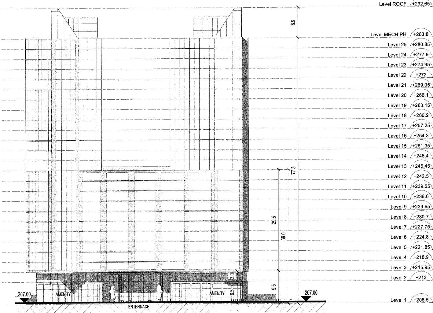
1 EAST ELEVATION 1 : 500
