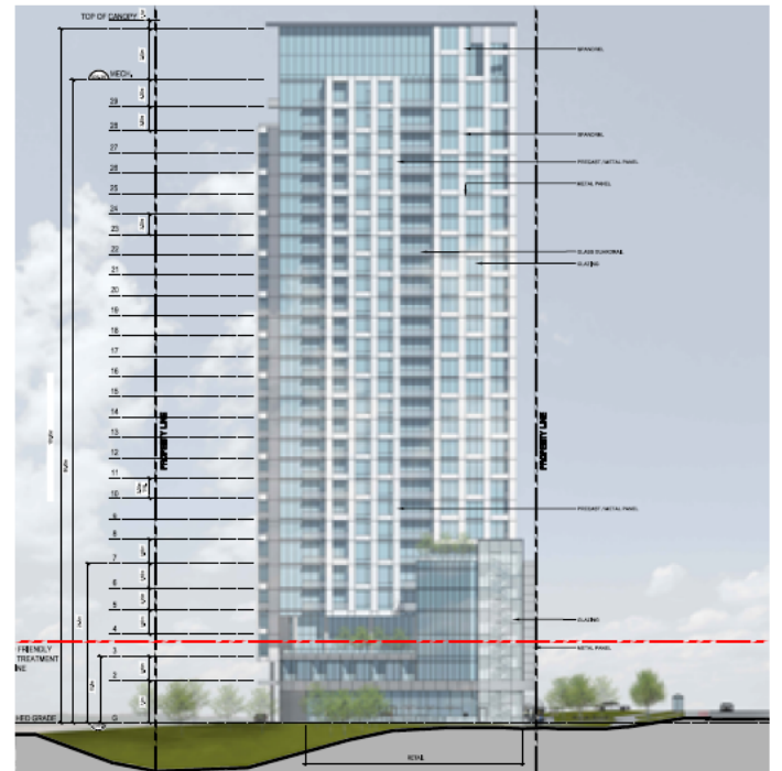
North Elevation (Kiwanis Memorial Park Frontage)
