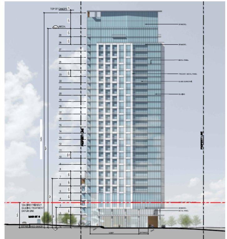
South Elevation (Bartley Bull Parkway Frontage)
