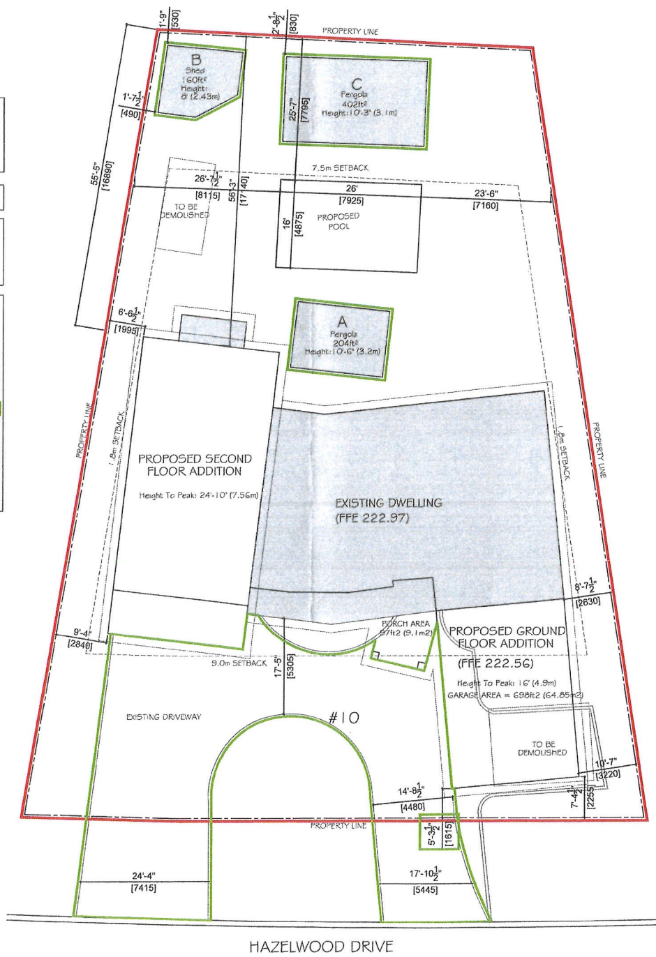
1 SITE PLAN 0.01 NTS JULY 15 / 2024
