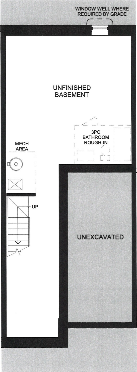
BASEMENT 695 ft 2
