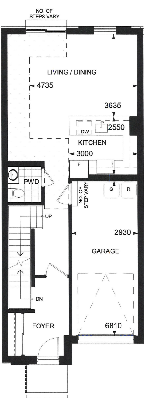
LEVEL 1 698 ft 2
