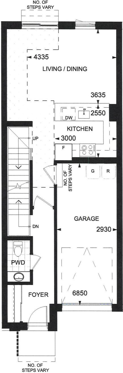
LEVEL 1 637 ft 2
