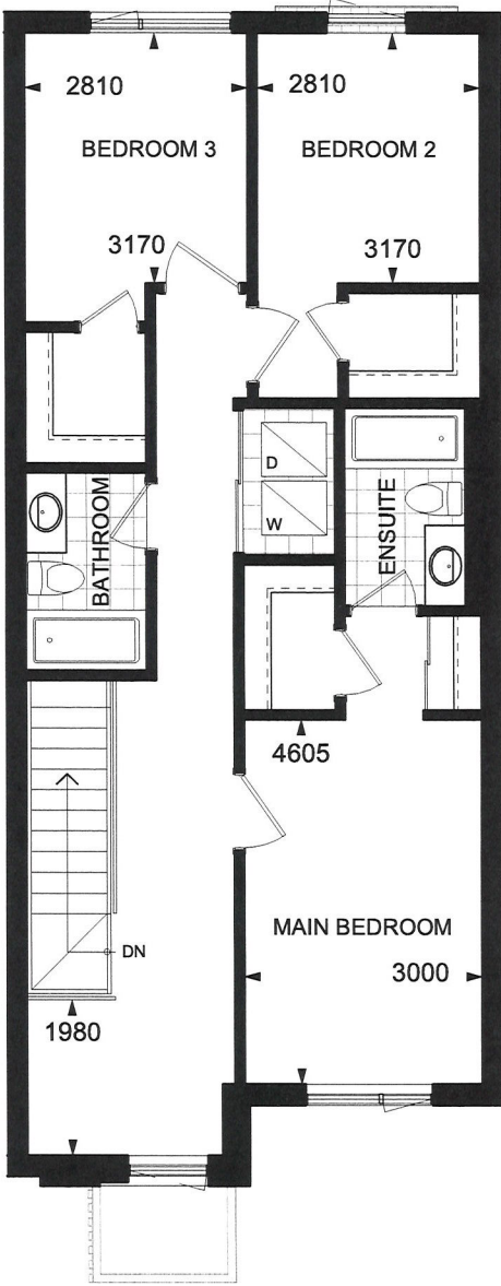
LEVEL 2 935 ft 2
