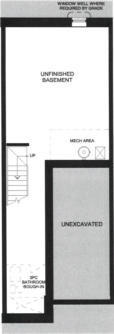
BASEMENT 693 ft 2
