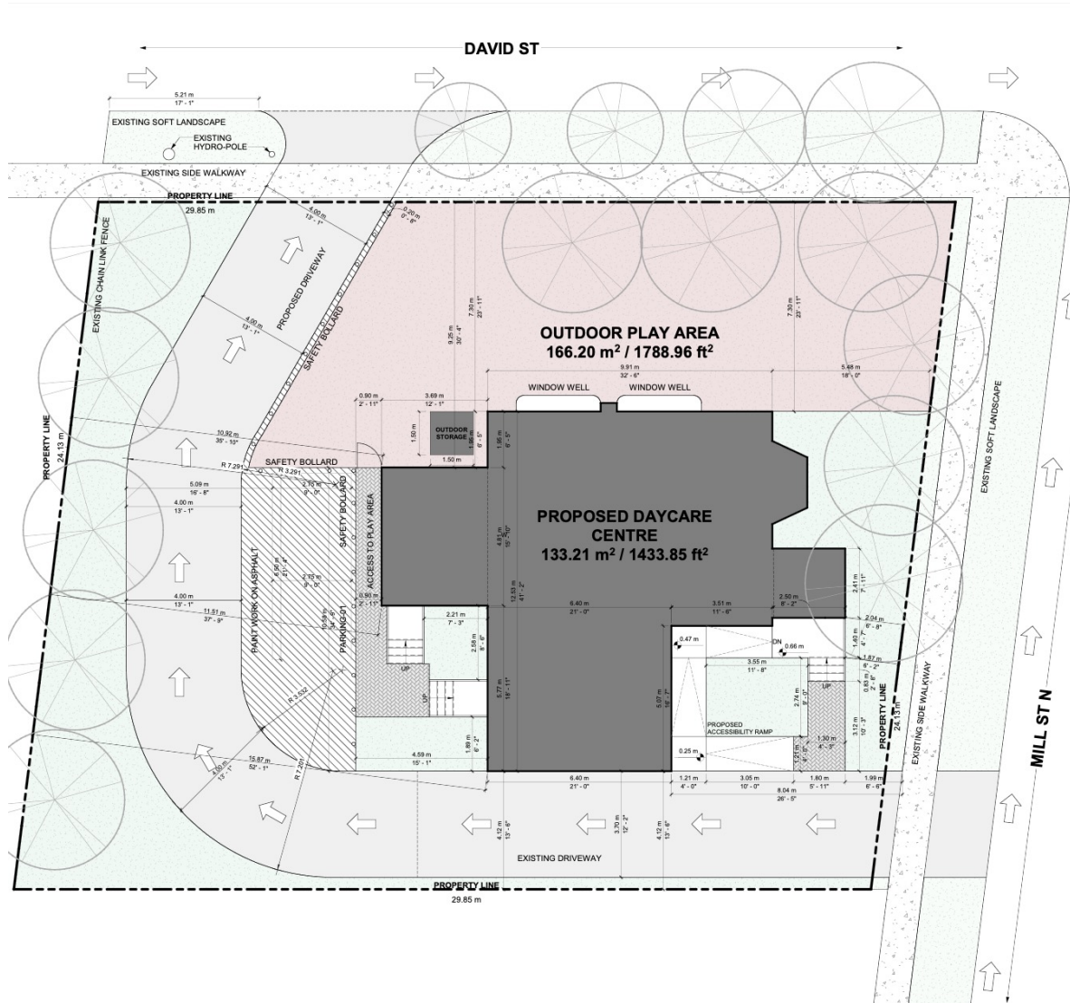
1 SITE PLAN - PROPOSED A0-002 1:84
