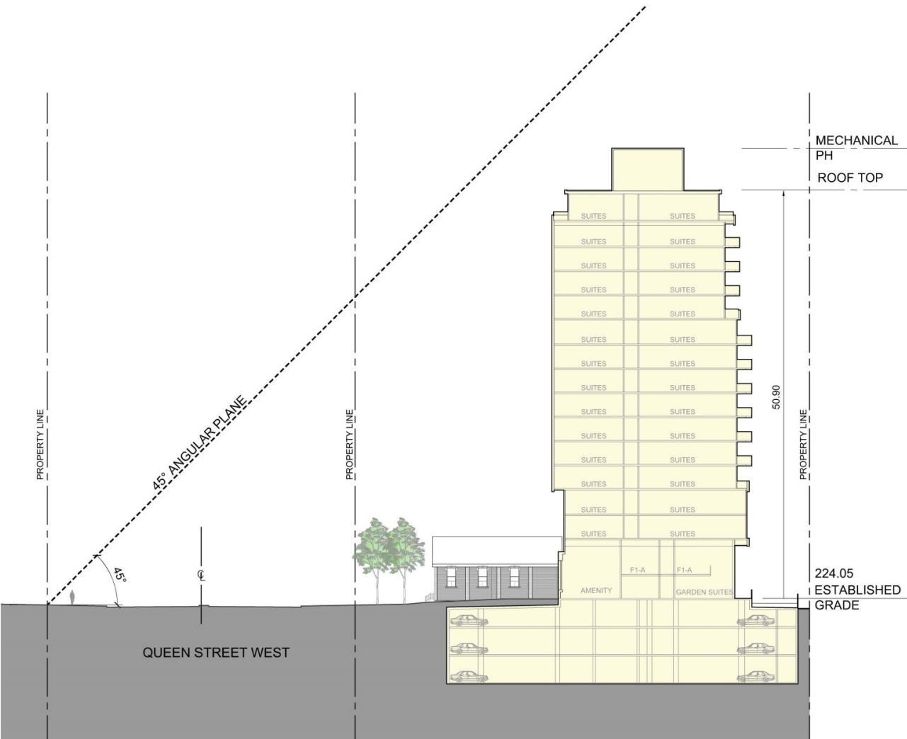
QUEEN STREET WEST CROSS-SECTION
