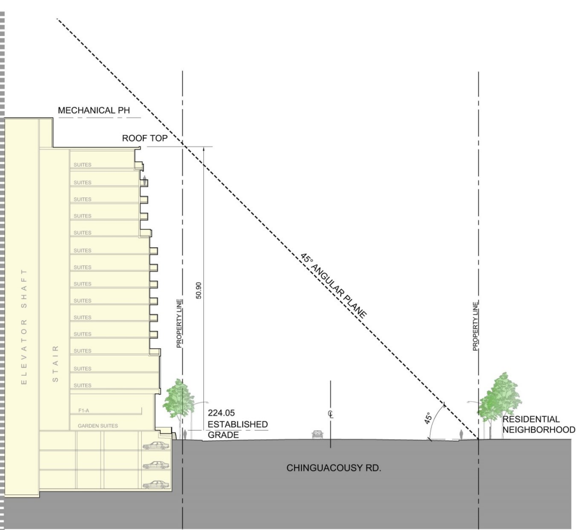
CHINGUACOUSY ROAD CROSS-SECTION
