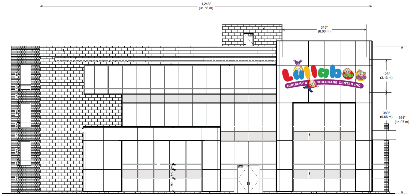
South Elevation
