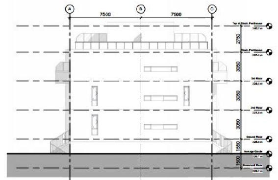
④ South Elevation - Block C 1 : 100
