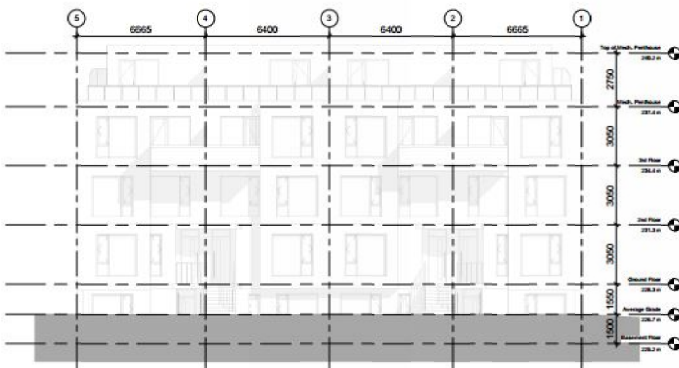
③ West Elevation - Block C 1 : 100
