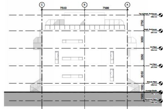
② North Elevation - Block C 1 : 100
