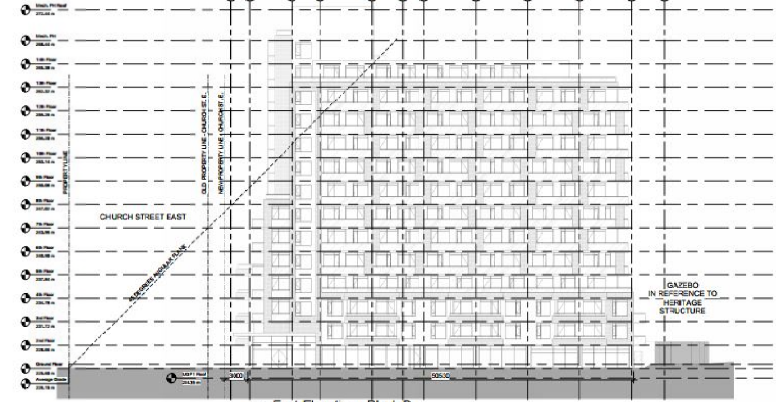
2 East Elevation - Block D 1:300
