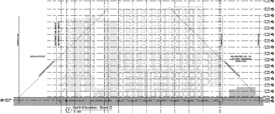
2 North Elevation - Block D 1:200
