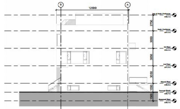
② East Elevation - Block A 1 : 100
