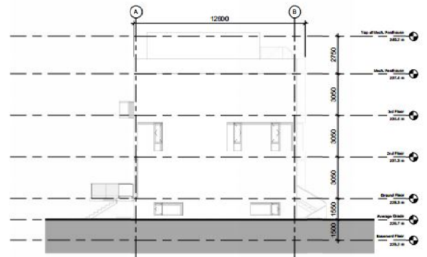
④ West Elevation - Block A 1 : 100
