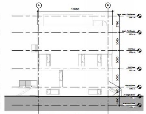
④ West Elevation - Block B 1 : 100
