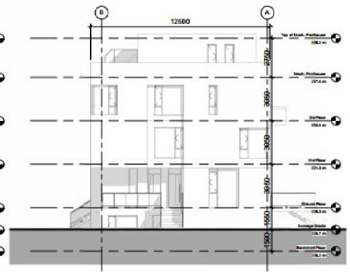
② East Elevation - Block B 1 : 100
