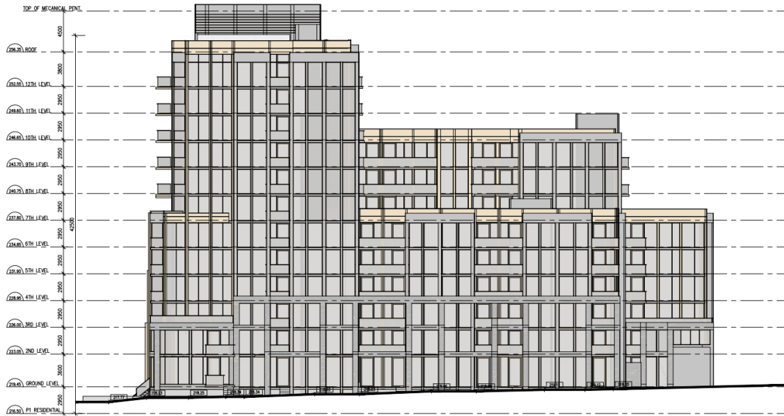
SOUTH-WEST ELEVATION (SIDE)
