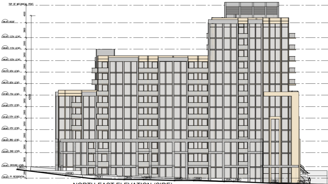
NORTH-EAST ELEVATION (SIDE)
